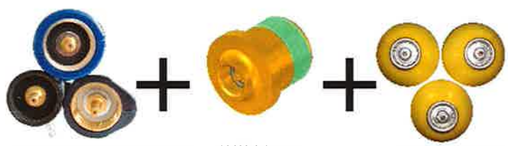
1" threaded US-Style torches. e.g. Rothenberger®, Turbo-Torch®, Monument 3440C 436U Adaptor Monument 434R GASEX®
